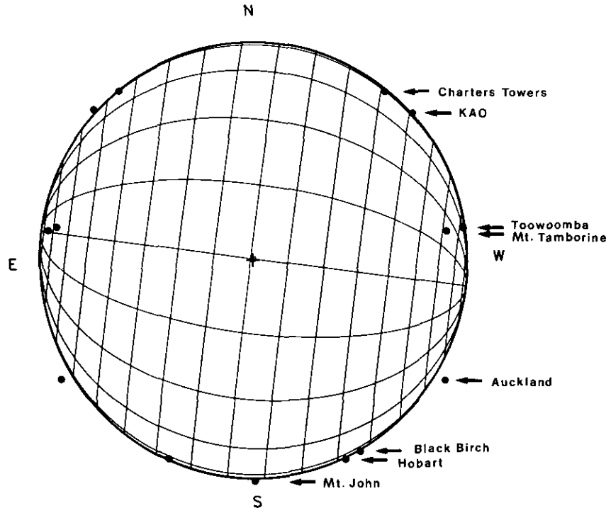
FIG. 3. A circle fitted by least squares to the observed points in Pluto's atmosphere corresponding to a 23.6% reduction of the light from P8. A latitude/longitude grid has been superimposed on the figure.
