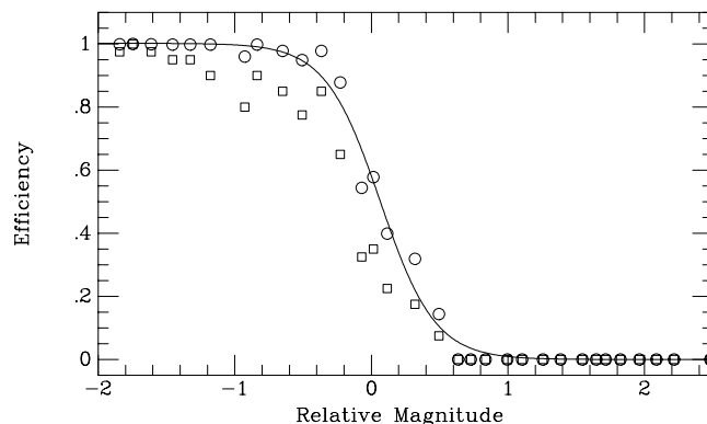
FIG. 4.—Efficiency of detection vs. relative apparent magnitude (limiting magnitude = 0). Squares represent the case in which the observations were scrutinized by the automatic detection software plus a single visual inspection of the images. Open circles indicate the results when two individuals independently scanned the images. The solid curve has been fitted to the open circles.
