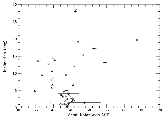
FIG. 11.—Inclination vs. semimajor axis for all objects discovered in the present investigation having uncertainties in semimajor axis less than 10 AU and which have received provisional MPC designations. Different symbols denote discoveries from different years as in Fig. 10.
