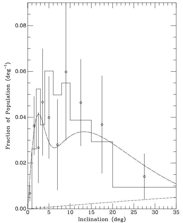
FIG. 13.—Inclination distribution for our sample of KBOs. The inclination distribution of our sample of KBOs with observational bias removed is shown by the open circles, for which the error bars have been determined from Poisson statistics. The units for the ordinate are given as the fraction of objects in the sample per degree of inclination. Our objects have been categorized into 1° bins from 0° to 4°, into 2° bins from 4° to 10°, and into 5° bins from 10° to 20° and a single bin from 20° to 35°. For reference, the inclination distribution of comets with periods less than 200 yr is shown by the solid histogram. Also for reference, we have plotted with alternating dots and dashes the \sin i distribution that would be expected from a distribution of orbits with poles in random directions. The dashed curve represents the inclination distribution derived by Brown (2001).
