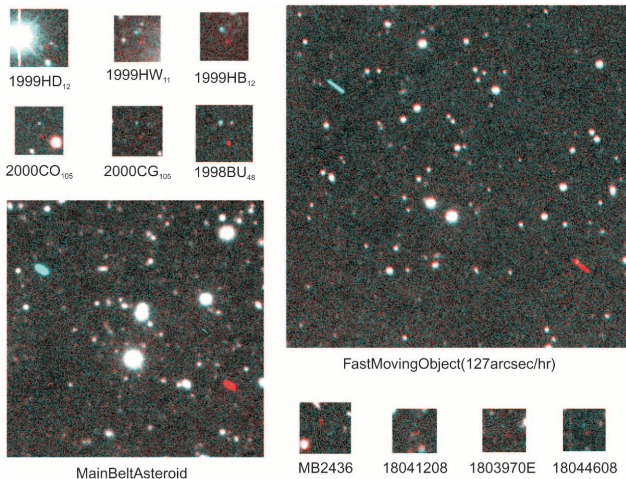
FIG. 3.—Sample images of moving objects as they appear with the detection technique described in this paper. Stationary objects appear white in the color images, while moving objects are seen as red-cyan pairs. The two larger squares illustrate the appearance of relatively rapidly moving objects such as main-belt asteroids. The smaller squares show the appearance of 10 objects or possible objects moving at rates appropriate to the Kuiper belt. Objects such as 1999 HB 12 and 1999 BU 48 are relatively bright and easy to find. Objects such as 2000 CG 105 are fainter but still readily detectable. 1803970E and 18044608 are near the limit at which we can detect moving objects with certainty, while 18041208 is perhaps at or below that limit. Observant readers will have noted that MB 2436, while quite bright, is moving in the opposite direction. This object is one of several enigmatic objects detected in the survey that we do not as yet have the resources to follow up.
