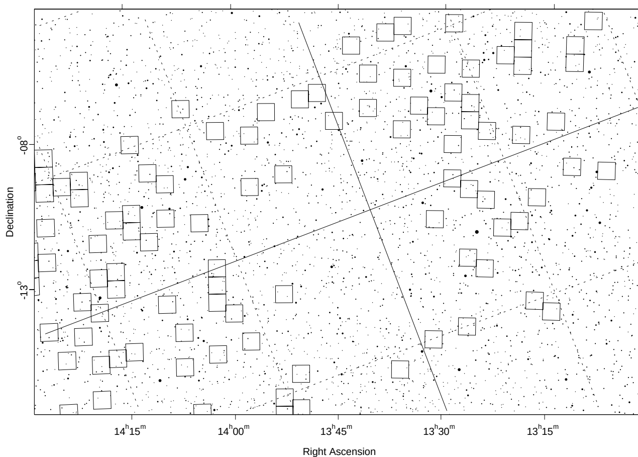
FIG. 2.—Sample map of search fields meeting the criteria of the Deep Ecliptic Survey. Each square is the size of a single Mosaic exposure. Declination is plotted along the ordinate, right ascension along the abscissa. The solid line running from lower left to upper right indicates the ecliptic. The intersection of the ecliptic with the other solid line indicates the location of the opposition point for the date of the chart. The dashed lines are spaced at intervals of 5°.
