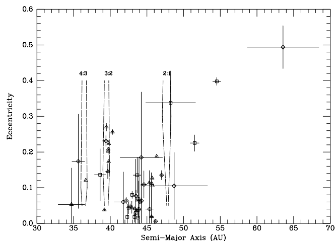
FIG. 12.—Eccentricity vs. semimajor axis for all objects discovered in the present investigation having uncertainties in semimajor axis less than 10 AU and which have received provisional MPC designations. Different symbols denote discoveries from different years as in Fig. 10. The dashed lines indicate the positions of various mean motion resonances with Neptune.
