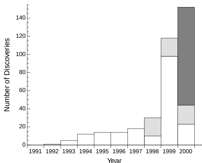
FIG. 1.—Number of KBOs that have received designations from the Minor Planet Center vs. year. The light gray segments indicate the observations discussed in this paper. The dark portion of the rightmost bar indicates KBOs discovered in 2000 after the cutoff date for data included in this paper.
