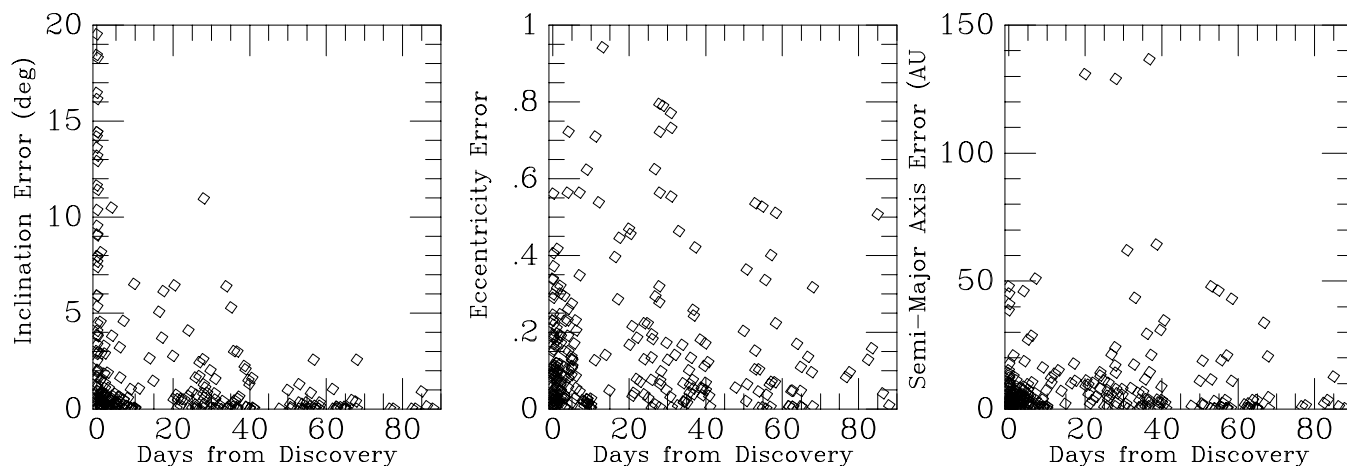
FIG. 7.—“Errors” in the orbital elements ( i , a , and e ) as a function of time from discovery of all KBOs known as of 2000 December 22 with astrometric observations extending over at least 2 yr. Individual points represent the difference between orbits determined by the method of Bernstein & Khushalani (2000) and the orbits from Bowell based on all available data.
