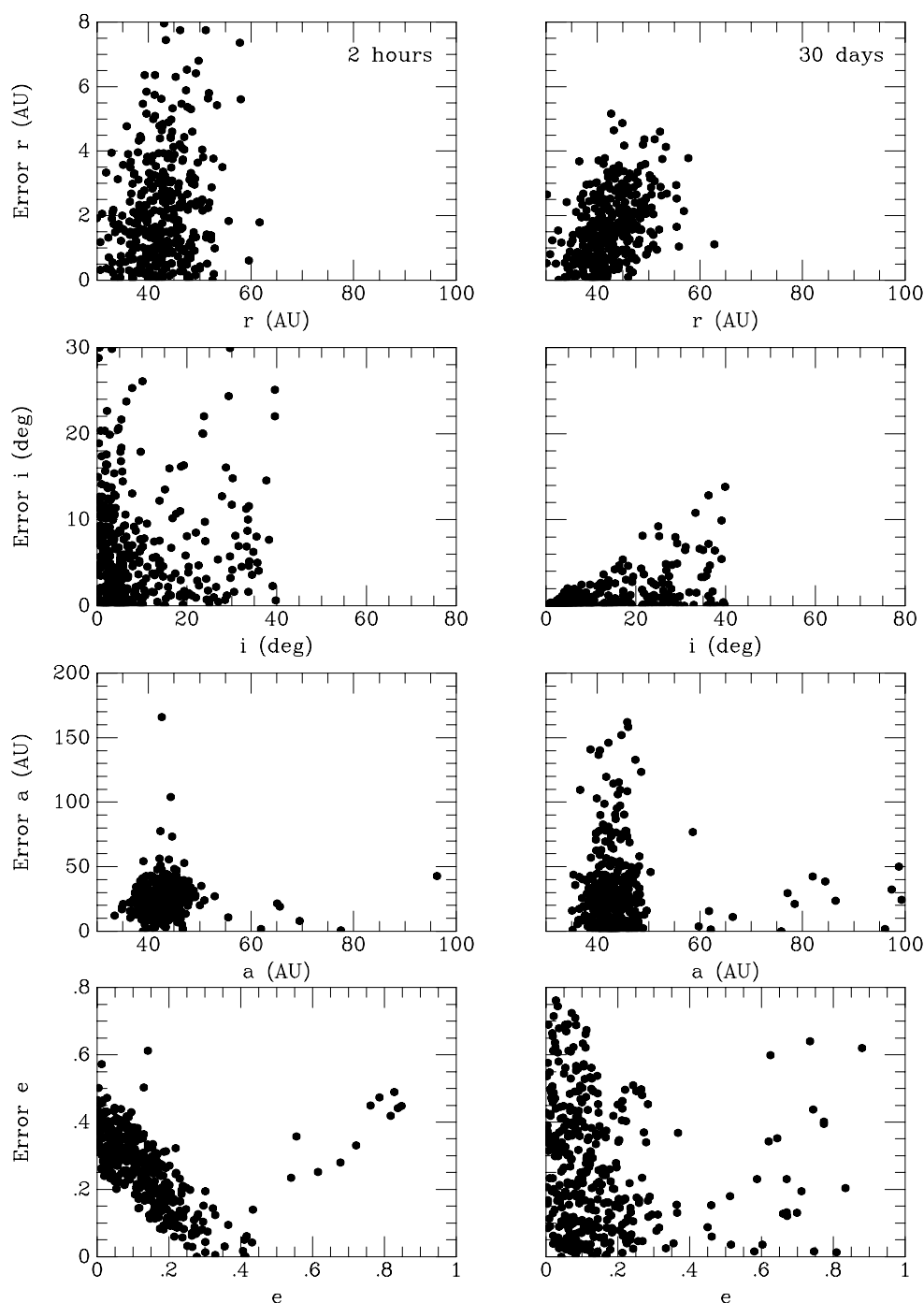
FIG. 5.—“Errors” in the calculated heliocentric distance, inclination, semimajor axis, and eccentricity of hypothetical KBO orbits as determined by the method of Väisälä (1939) for observational coverage spanning 2 hr, 30 days, 60 days, and 1 yr.
