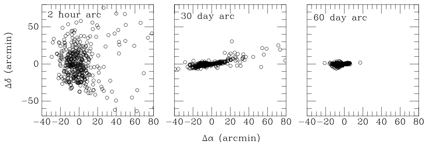
FIG. 8.—“Errors” in the predicted positions 1 year from the date of discovery of hypothetical KBOs with 2 hr, 30 day, and 60 day astrometric coverage. Predictions are based on orbits determined by the method of Bernstein & Khushalani (2000).
