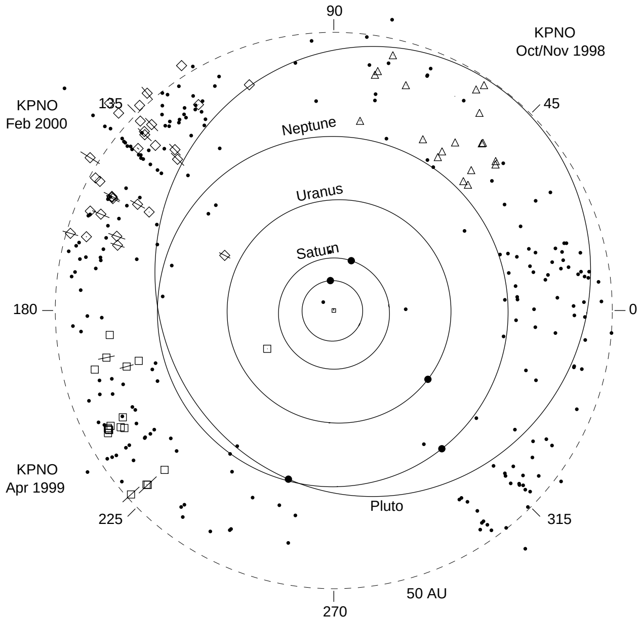
FIG. 10.—Distribution of KBOs and Centaurs discovered in this survey vs. heliocentric distance (projected onto the plane of the ecliptic) and ecliptic longitude. Triangles denote objects discovered in 1998; squares were discovered in 1999, and diamonds are objects found in 2000. Also shown are the orbits and positions of the five outer planets. The dashed circle has a radius of 50 AU. Small filled circles indicate the positions of other known KBOs.
