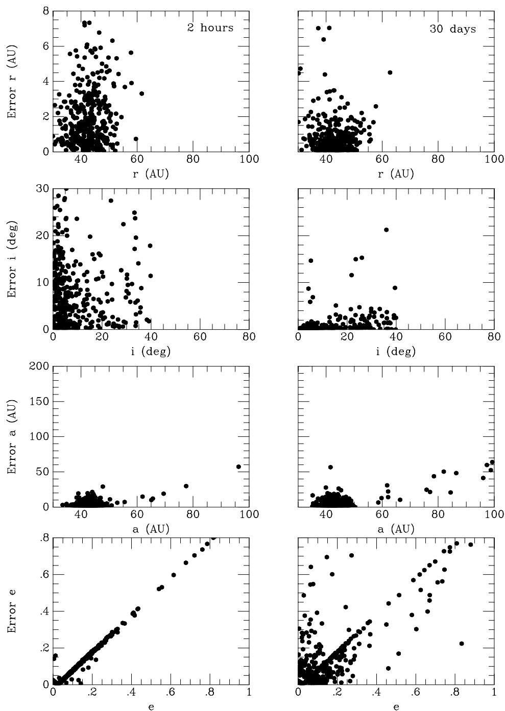
FIG. 6.—“Errors” in the calculated heliocentric distance, inclination, semimajor axis, and eccentricity of hypothetical KBO orbits as determined by the method of Bernstein & Khushalani (2000) for observational coverage spanning 2 hr, 30 days, 60 days, and 1 yr.
