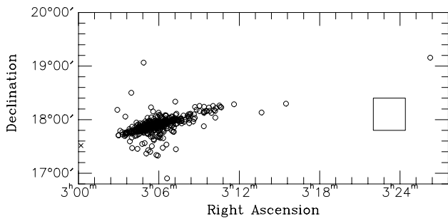
FIG. 9.—Annual motion of KBOs. The cross indicates the initial position of a population of hypothetical objects in KBO-like orbits forced by adjustment of the mean anomaly to fall within a 30'' \times 30'' box on the sky. After 1 yr, these objects would be found at the positions indicated by open circles. The square indicates the area covered by a single Mosaic exposure.
